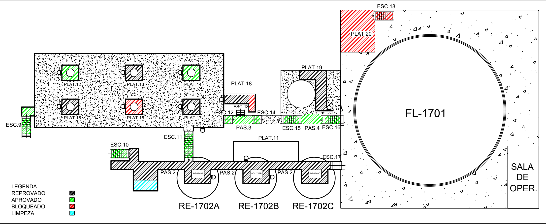
DESENHO 11.3 - RE-1702A / RE-1702B / RE-1702C - 3° PATAMAR
